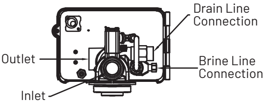
BACK VIEW OF 2850 CONTROL VALVE
